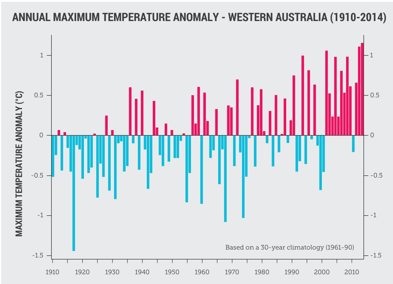
Figure 3: Western Australia is experiencing a long-term increase in annual maximum temperatures. Magenta bars indicate years of above average maximum temperatures (Adapted from BoM 2015c).
